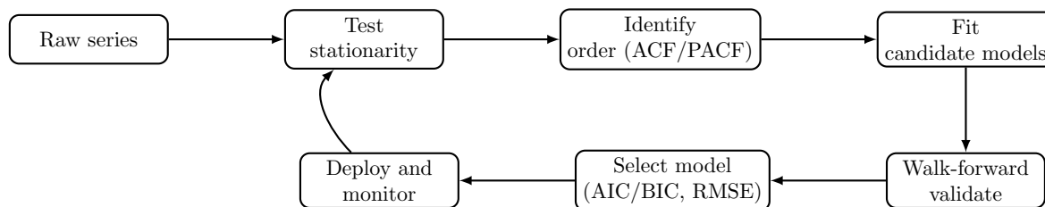
Figure 1.4: A practical time series modeling workflow: test stationarity, identify candidate model orders, fit several candidates, validate with a walk-forward scheme, select the best model, and monitor after deployment, periodically revisiting earlier steps as new data arrives.
