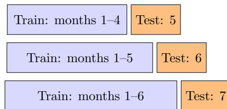
Figure 1.3: Walk-forward validation: the training window always ends before the test period, and both roll forward together, so no forecast ever uses future information.
