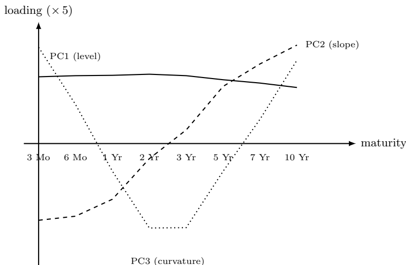
Figure 1.2: PCA loadings by maturity for the first three principal components of the 1990–2023 Treasury yield curve panel. PC1 loads almost equally and positively on every maturity (a parallel shift, or level factor); PC2 loads negatively on short maturities and positively on long ones (a steepening or flattening, or slope factor); PC3 loads positively at both ends and negatively in the middle (a curvature or “butterfly” factor).
