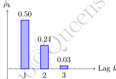
Figure 1.1: Sample correlogram for the interest-rate deviation series in Table 1.1. The roughly geometric decay is characteristic of an AR(1) process.
