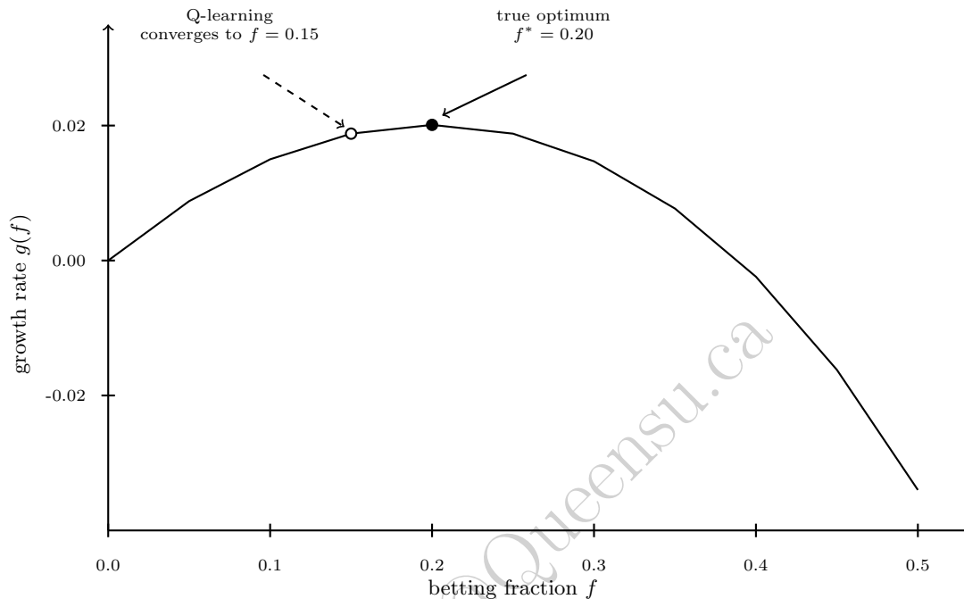
Figure 19.6: The Kelly growth-rate curve g(f) = p \ln(1 + f) + q \ln(1 - f) for p = 0.6 , b = 1 .
