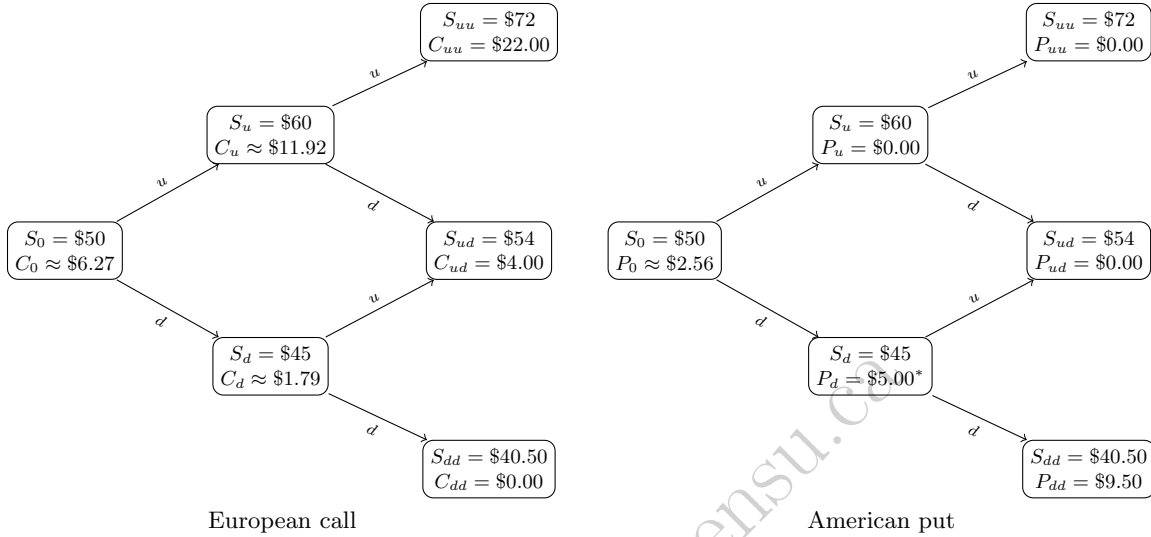
Figure 5.2: The two-step binomial tree for the $50-strike European call (left) and American put (right). Both share the same stock-price tree, growing forward from S_0 under up- and down-moves u = 1.2 and d = 0.9 and recombining at the middle terminal node. Option values (bottom line of each node) are computed backward from the known terminal payoffs using the risk-neutral probability q = 0.467 , except at the American put's down node, marked with an asterisk, where the $5.00 intrinsic value of immediate exercise replaces the lower $4.87 continuation value, producing the early-exercise premium discussed in the text.
