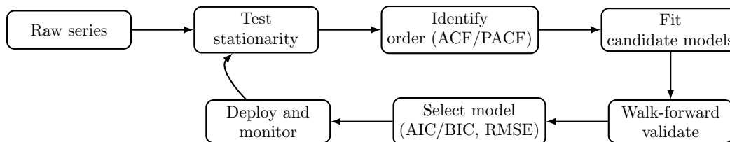
Figure 7.4: A practical time series modeling workflow.
