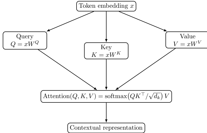
Figure 16.2: The self-attention computation as a diagram.
