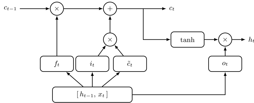
Figure 17.4: The LSTM cell. The cell state crosses the top of the diagram scaled once and added to once, never passed through a squashing function, which is why information survives along it; the three gates below all read the same concatenated [h_{t-1}, x_t] .
