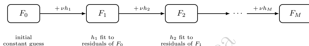
Figure 1.8: Gradient boosting as a sequential chain. The ensemble prediction F_m is built by adding a shrunk new tree \nu h_m to the previous stage F_{m-1} , where h_m is fit to correct whatever F_{m-1} still gets wrong. Each stage depends on every stage before it, unlike the independently-grown, averaged trees of a random forest summarized in Table 1.9.
