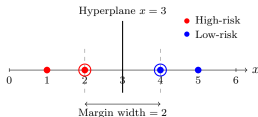
Figure 1.4: The maximum-margin hyperplane for the one-dimensional example: two high-risk points ( x = 1, 2 ) and two low-risk points ( x = 4, 5 ). The support vectors ( x = 2 and x = 4 , circled) alone determine the hyperplane at x = 3 and the margin boundaries (dashed) on either side of it; the points at x = 1 and x = 5 play no role and could move freely without changing the boundary.
