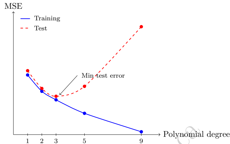
Figure 1.5: Training and test error (MSE) from Table 1.6 as polynomial degree increases. Training error falls monotonically as the model gains flexibility, but test error is minimized at degree 3 and rises sharply beyond it, the signature of overfitting once the model becomes flexible enough to fit noise in the training sample.
