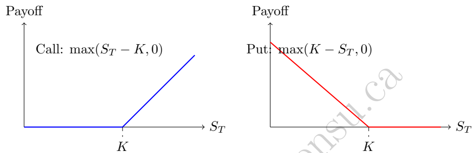
Figure 5.1: Payoff at maturity for a call option (left) and a put option (right) with strike K
