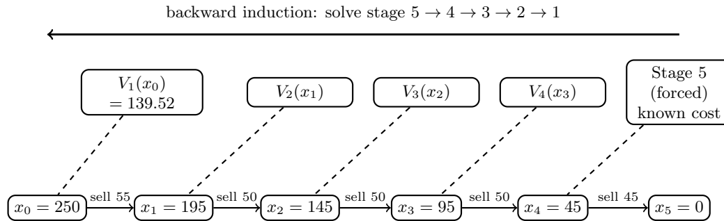
Figure 19.4: Backward-induction dynamic programming for the execution problem
