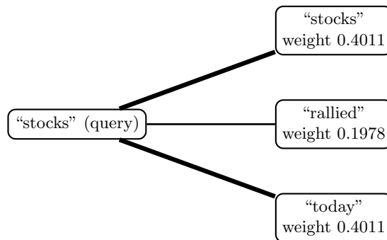
Figure 16.3: Self-attention weights for the query token “stocks” over the three-token sentence “stocks rallied today,” with edge thickness proportional to attention weight
