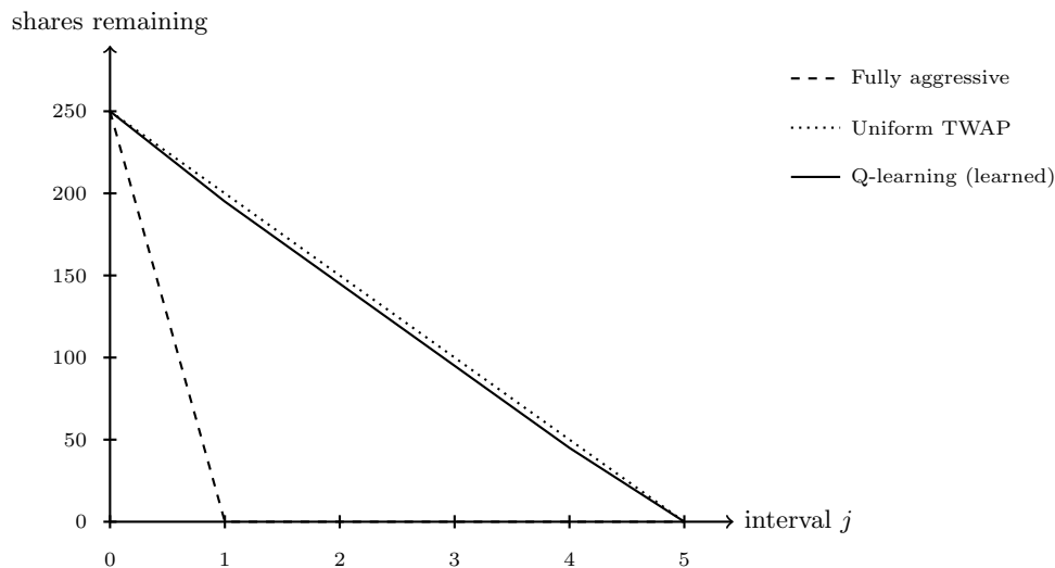
Figure 19.5: Unexecuted-share trajectories under the three strategies of Table 19.4
