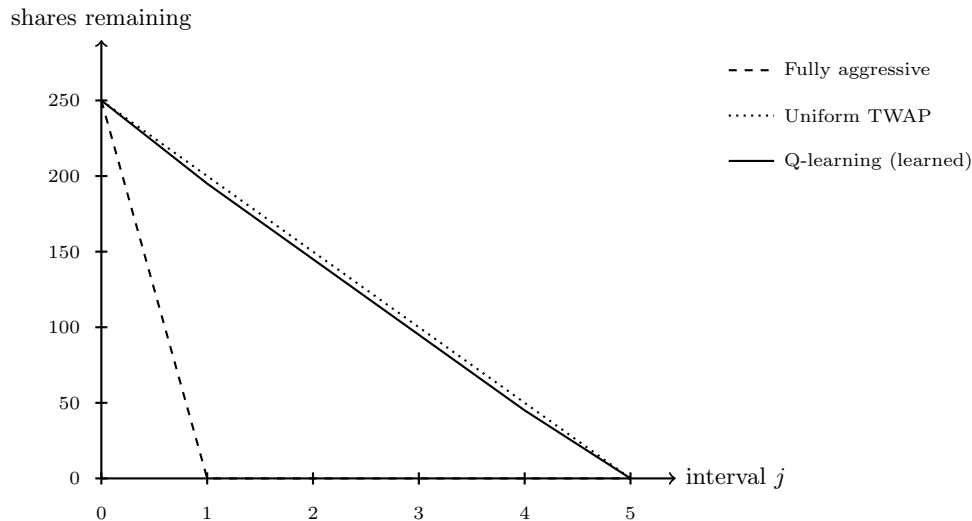
Figure 1.5: Unexecuted-share trajectories under the three strategies of Table 1.4
