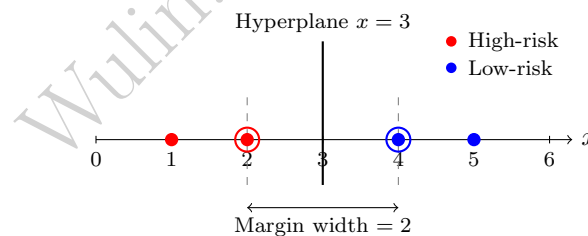
Figure 1.4: The maximum-margin hyperplane for the one-dimensional example: two high-risk points ( x = 1, 2 ) and two low-risk points ( x = 4, 5 ), with the support vectors circled
