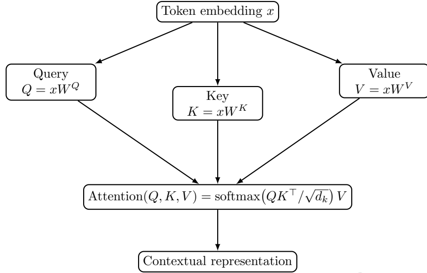
Figure 1.2: The self-attention computation as a diagram.
