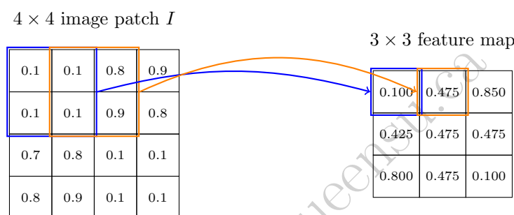
Figure 15.2: Sliding a 2 \times 2 averaging filter across the 4 \times 4 satellite patch I at stride 1. The blue-highlighted patch (the top-left 2 \times 2 block) averages to 0.100; sliding the filter one column right, the orange-highlighted patch averages to 0.475, the two feature-map entries worked out in the text. Repeating this for all nine filter positions produces the full 3 \times 3 feature map, with the two car-cluster corners (0.850, 0.800) standing out clearly from the two empty corners (both 0.100).
