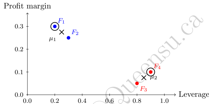
Figure 6.6: The K -means example: four firms in leverage/profit-margin space, colored by their converged cluster assignment (blue: low-leverage, higher-margin; red: high-leverage, low-margin). Circled points mark the two initial centers (placed at F_1 and F_4 ); the \times markers show the updated centers \mu_1 and \mu_2 after one iteration, at which point the algorithm has converged.
