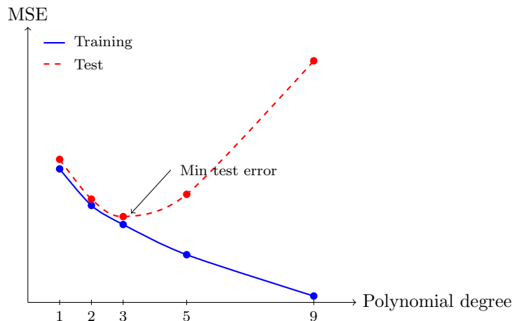
Figure 6.3: Training and test error (MSE) from Table 6.5 as polynomial degree increases. Training error falls monotonically as the model gains flexibility, but test error is minimized at degree 3 and rises sharply beyond it, the signature of overfitting once the model becomes flexible enough to fit noise in the training sample.
