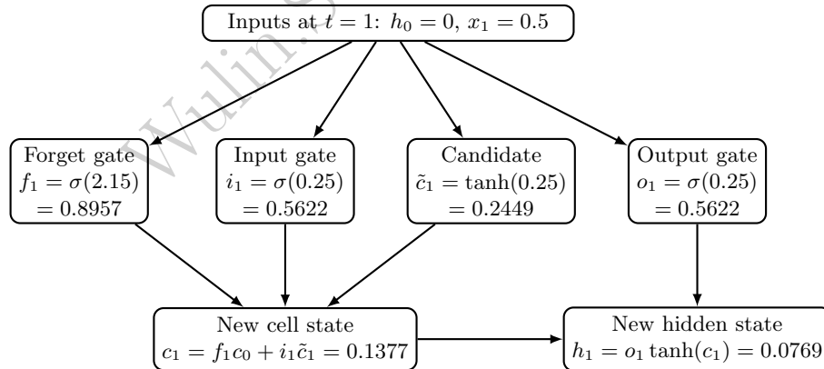
Figure 15.4: The LSTM cell's first time step, computed from the worked example in the text. All four gates, forget, input, candidate, and output, are computed from the same inputs ( h_0, x_1 ); the forget and input gates combine with the candidate value to produce the new cell state c_1 , and the output gate then determines how much of c_1 (passed through \tanh ) becomes the new hidden state h_1 .
