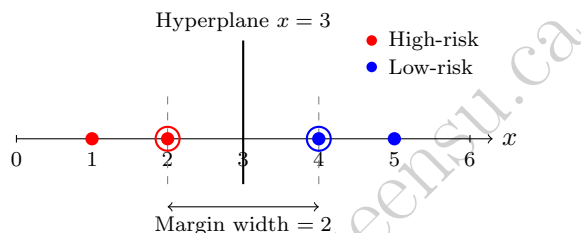
Figure 6.2: The maximum-margin hyperplane for the one-dimensional example: two high-risk points ( x = 1, 2 ) and two low-risk points ( x = 4, 5 ). The support vectors ( x = 2 and x = 4 , circled) alone determine the hyperplane at x = 3 and the margin boundaries (dashed) on either side of it; the points at x = 1 and x = 5 play no role and could move freely without changing the boundary.
