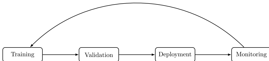
Figure 6.5: A machine learning workflow in finance should include training, validation, deployment, and continuous monitoring, with findings from monitoring feeding back into retraining.
