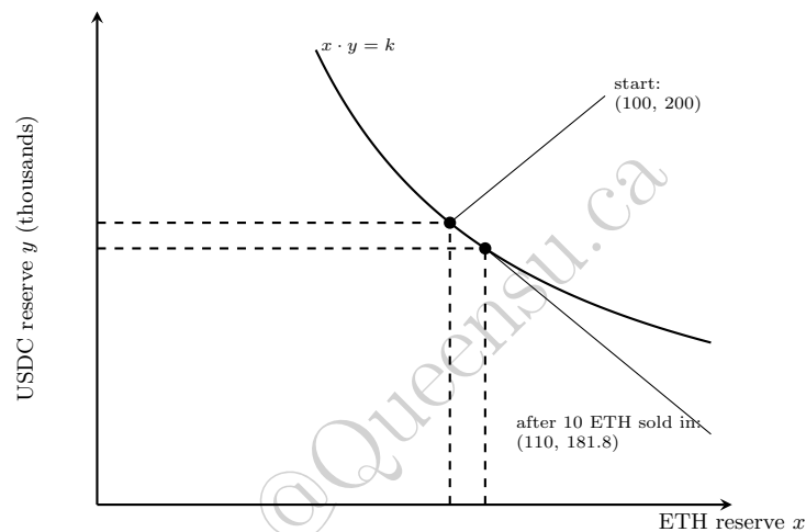
Figure 13.3: The constant-product curve x \cdot y = k . Selling ETH into the pool moves the pool's reserves down and to the right along the curve; the curvature is what generates price impact directly from the trade size, with no order book involved.
