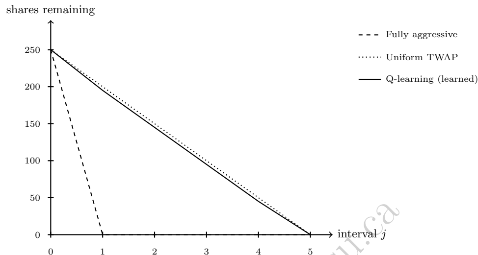
Figure 17.5: Unexecuted-share trajectories under the three strategies of Table 17.3.
