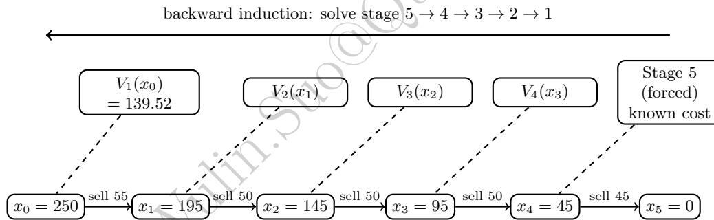
Figure 17.4: Backward-induction dynamic programming for the execution problem.
