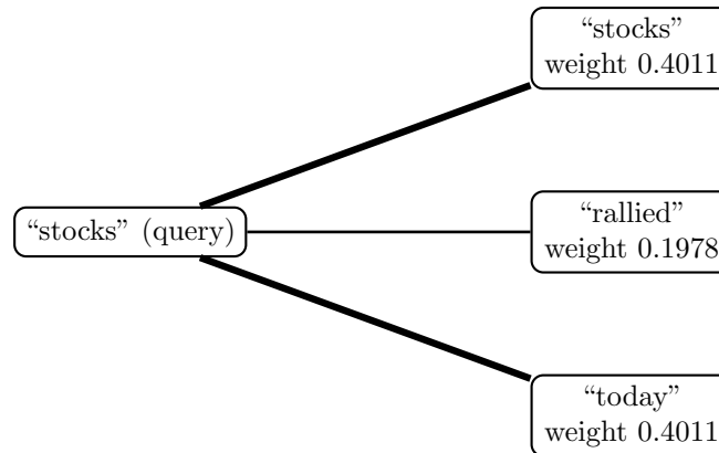
Figure 14.3: Self-attention weights for the query token “stocks” over the three-token sentence “stocks rallied today,” with edge thickness proportional to attention weight.
