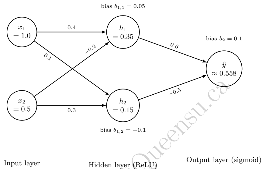
Figure 6.10: The toy feedforward network worked through above. Chapter 16 revisits it to verify LIME and integrated-gradients explanations against its exact analytical gradient.
