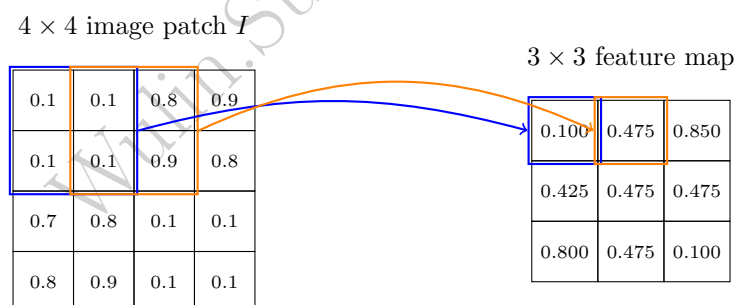
Figure 15.2: Sliding a 2 \times 2 averaging filter across the 4 \times 4 satellite patch I at stride 1.
