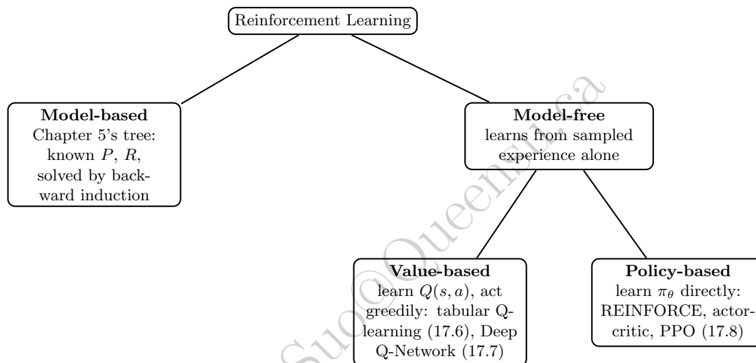
Figure 17.2: A map of the reinforcement learning methods this chapter develops.
