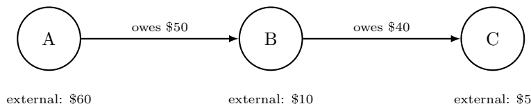
Figure 18.2: A three-bank interbank obligation network.
