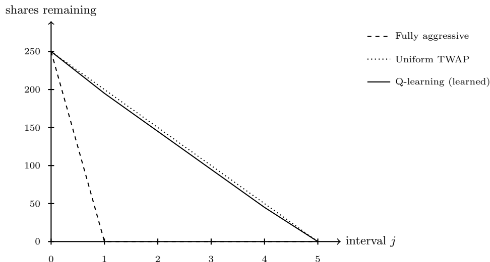
Figure 17.5: Unexecuted-share trajectories under the three strategies of Table 17.3.
