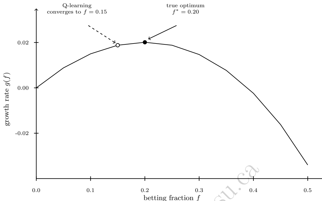
Figure 17.6: The Kelly growth-rate curve g(f) = p \ln(1 + f) + q \ln(1 - f) for p = 0.6 , b = 1 .
