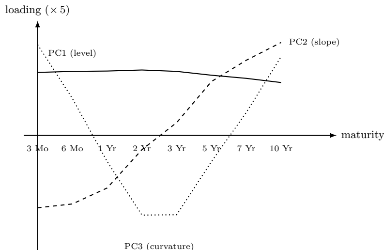
Figure 7.2: PCA loadings by maturity for the first three principal components of the 1990–2023 Treasury yield curve panel.
