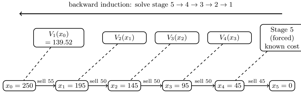
Figure 17.4: Backward-induction dynamic programming for the execution problem.
