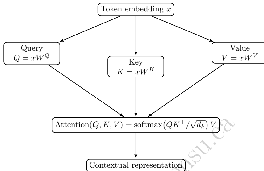
Figure 14.2: The self-attention computation as a diagram.
