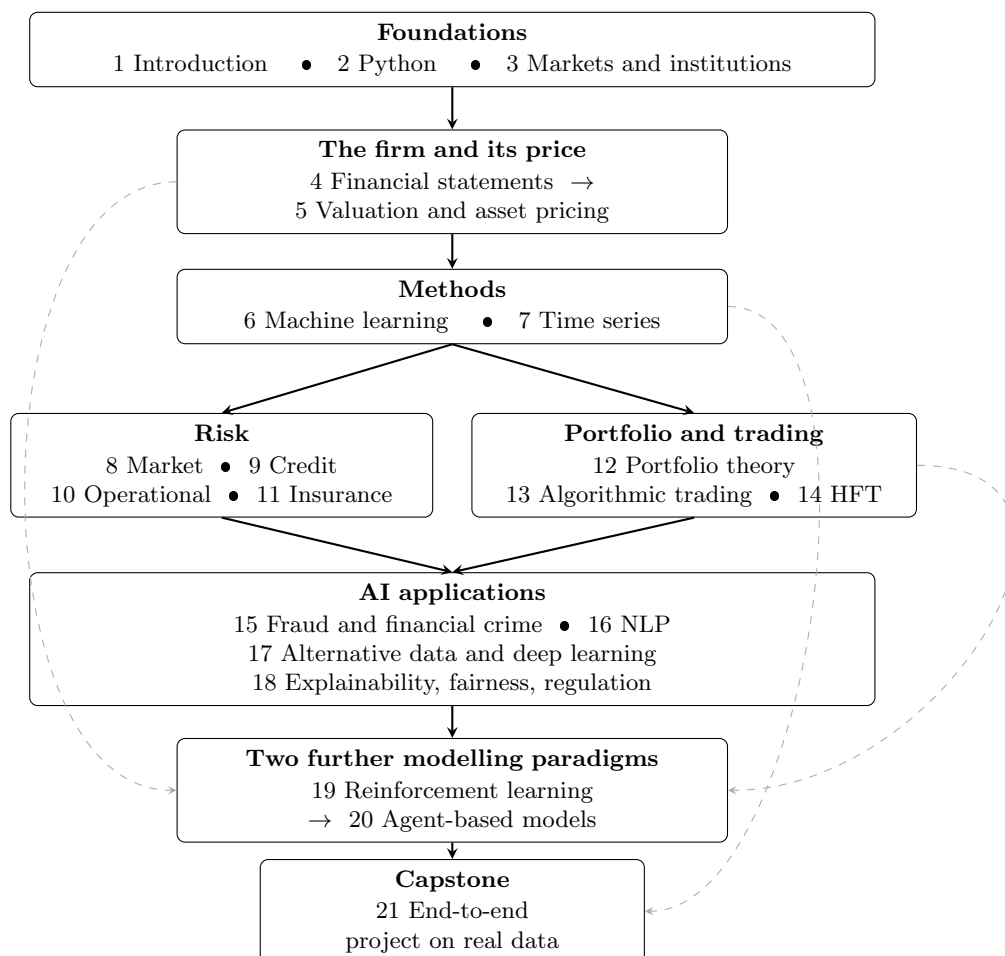
Figure 1: How the chapters depend on one another. Solid arrows are prerequisites. The three dashed arrows mark the places where a later group reuses an earlier one's machinery rather than rebuilding it: Chapter 5's option pricing returns in Chapters 8, 9, 12, and 19; Chapter 6's models are reused by Chapter 9 and Chapters 15 through 18 rather than retaught; and Chapter 13's execution model returns in Chapter 19. Chapter 2 underpins every companion notebook in the book and Chapter 21 draws on all of it, so neither is drawn with an arrow to each dependent chapter. An instructor short of sessions can cut most safely within a group rather than across the spine.
