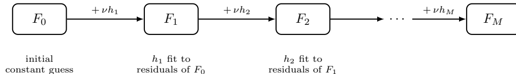
Figure 6.8: Gradient boosting as a sequential chain of shrunk trees, each fit to correct the previous stage's residuals
