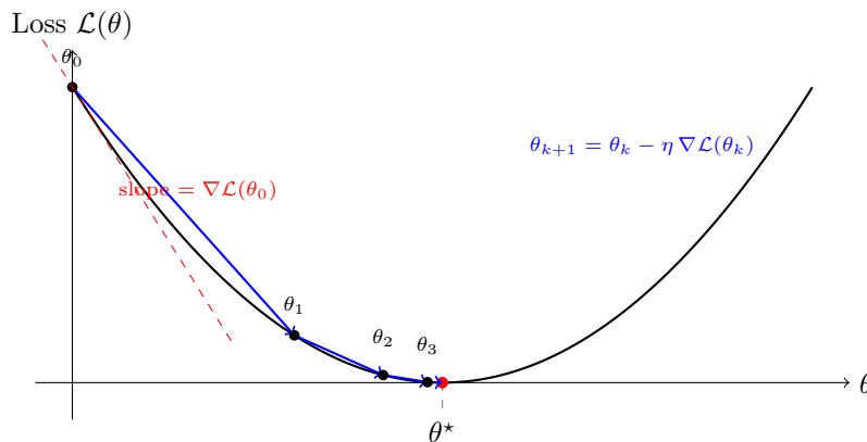
Figure 6.2: The idea of gradient descent. Starting from an initial guess \theta_0 , each step moves against the local slope of the loss curve, the negative gradient, illustrated here by the tangent line at \theta_0 , producing a sequence \theta_0, \theta_1, \theta_2, \dots that descends toward the minimizer \theta^* . Steps are large where the curve is steep and shrink automatically as the curve flattens near the minimum, the pattern seen numerically in Table 6.2 below.
