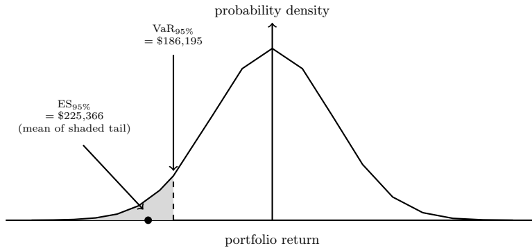
Figure 1.1: The parametric VaR and Expected Shortfall of Table 1.2's portfolio, illustrated against the assumed normal return distribution
