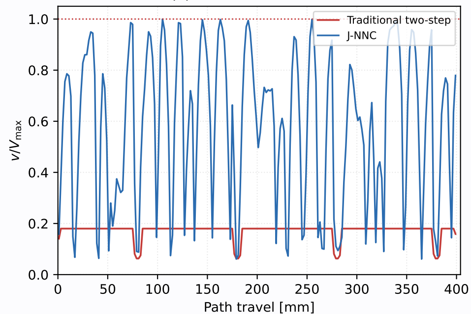
(c) Feedrate utilization
