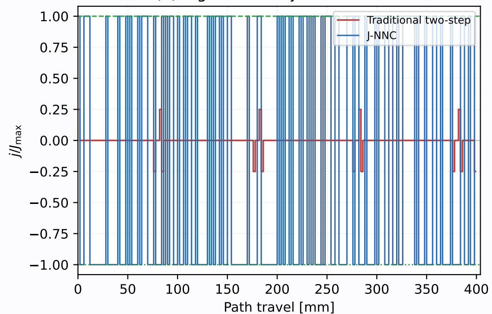
(d) Signed linear jerk utilization
