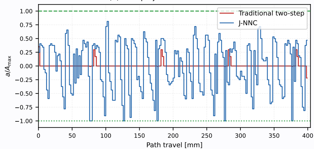
(e) KCM-projected linear-jerk use
