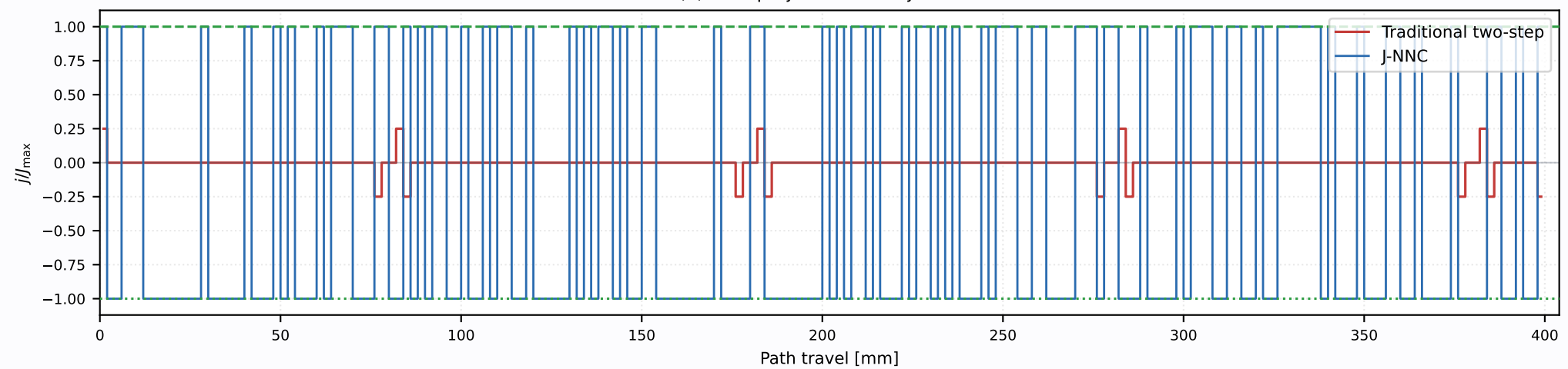
(e) KCM-projected linear-jerk use
