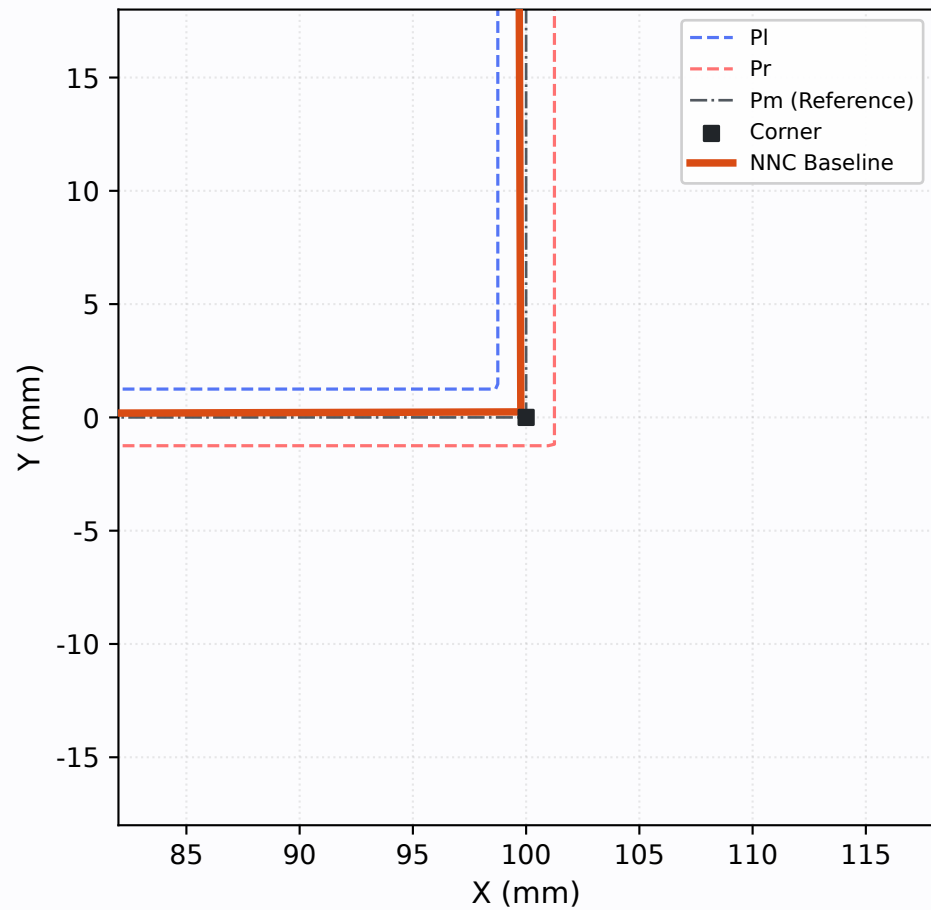
NNC Baseline
