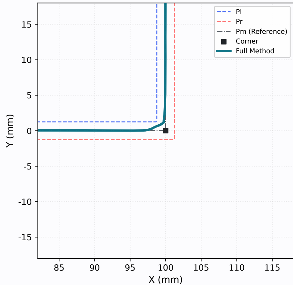
Full Method
