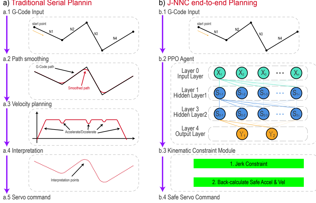
Figure 1: Comparison between conventional serial motion planning and the J-NNC motion-planning framework. J-NNC denotes the Jerk-constrained Neural Numerical Controller, i.e., a neural-network-based CNC motion planner with jerk-constrained action projection.
