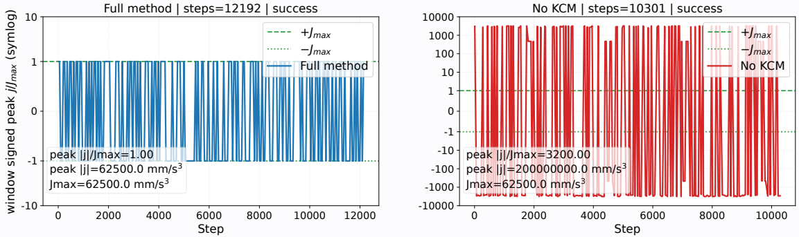
Figure 7: Comparison of linear jerk and jerk constraints between the final method proposed in this paper and the configuration without KCM on the same representative path.
