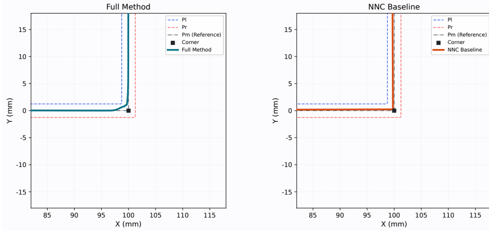
Figure 5: Local zoomed-in comparison of the trajectories generated by the proposed method and the NNC method in the corner region of the square path.
