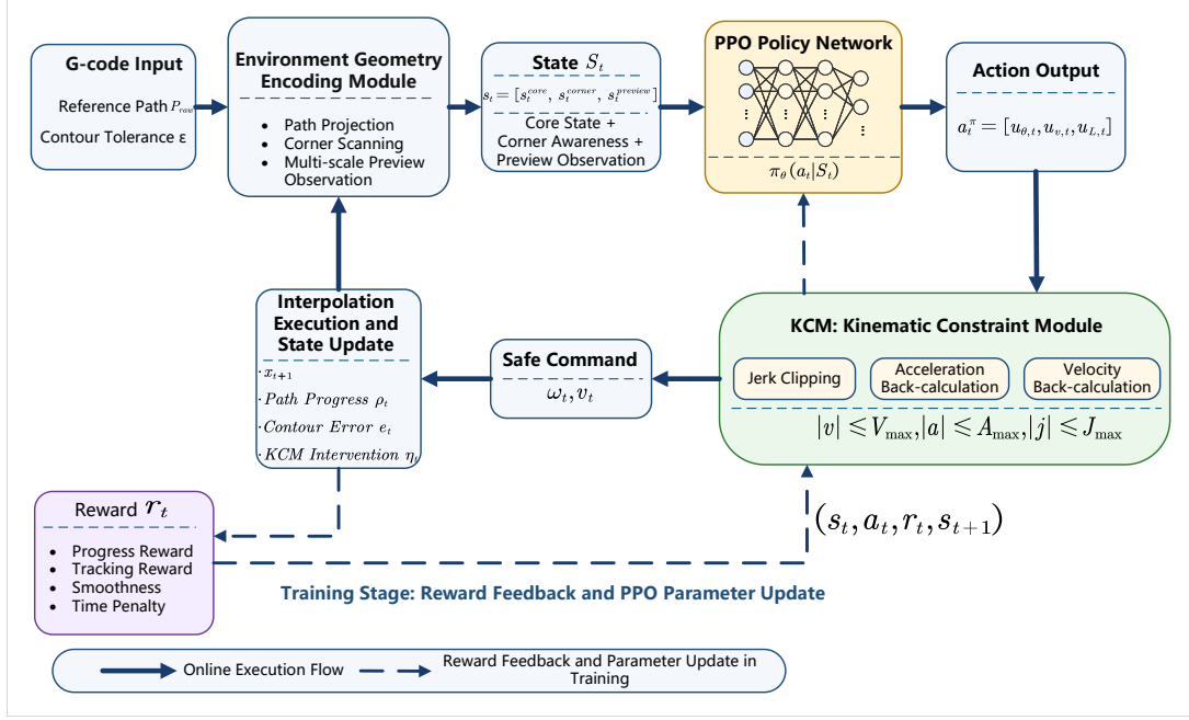
Figure 3: Overall closed-loop framework of the proposed method.
