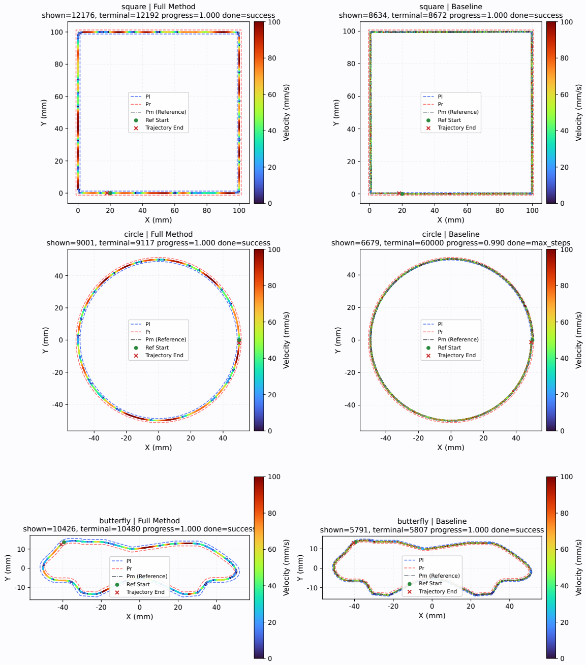
Figure 4: Trajectory comparison between the proposed method and the baseline methods in representative path scenarios.
