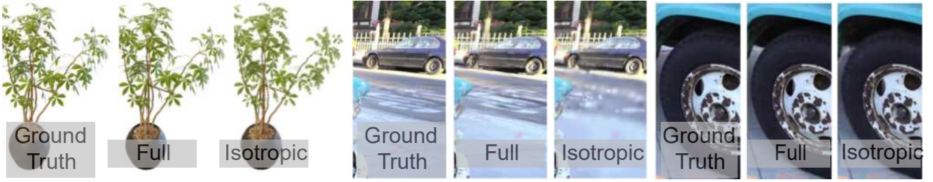
Fig. 10. We train scenes with Gaussian anisotropy disabled and enabled. The use of anisotropic volumetric splats enables modelling of fine structures and has a significant impact on visual quality. Note that for illustrative purposes, we restricted Ficus to use no more than 5k Gaussians in both configurations.
