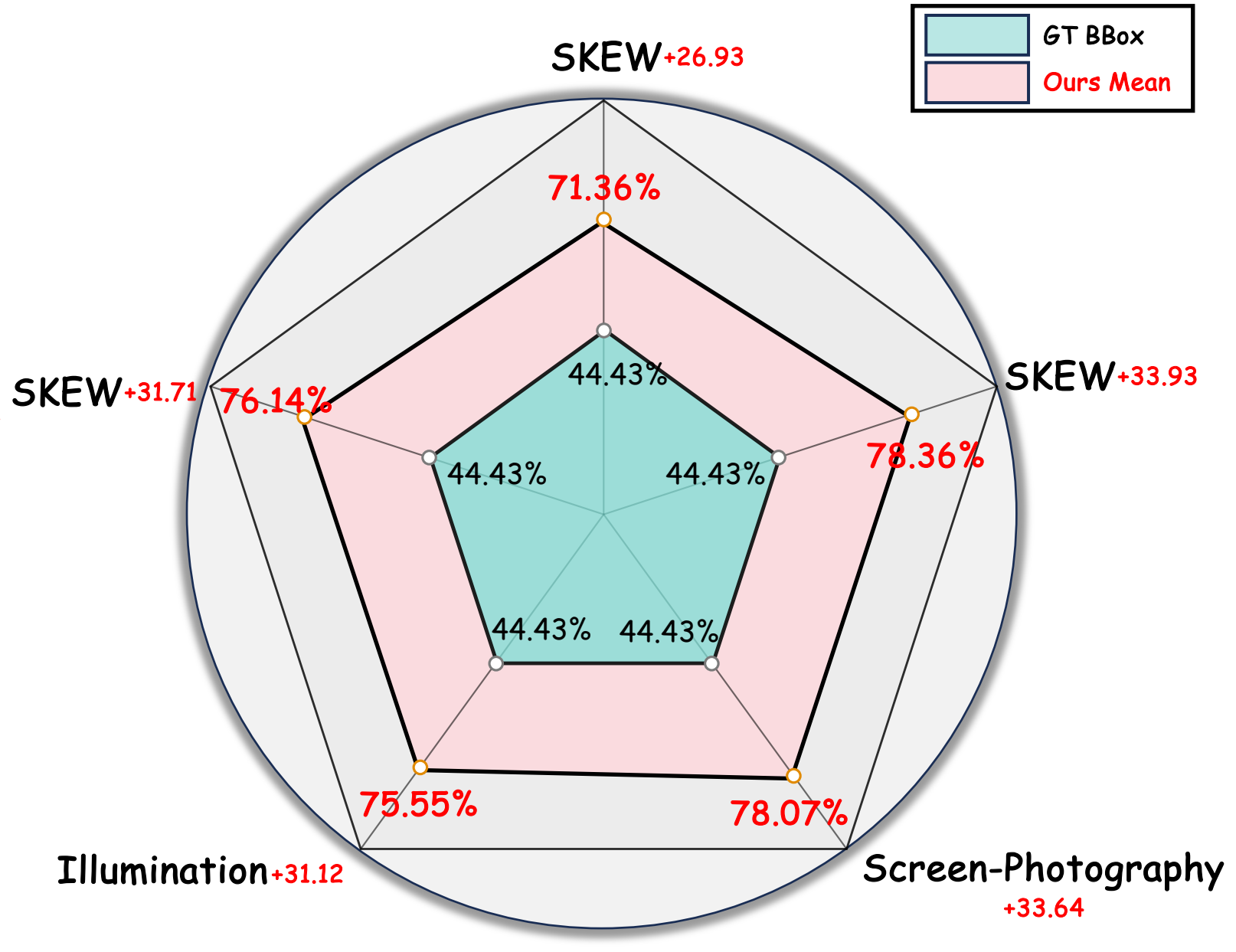
Real5-OmniDocBench
