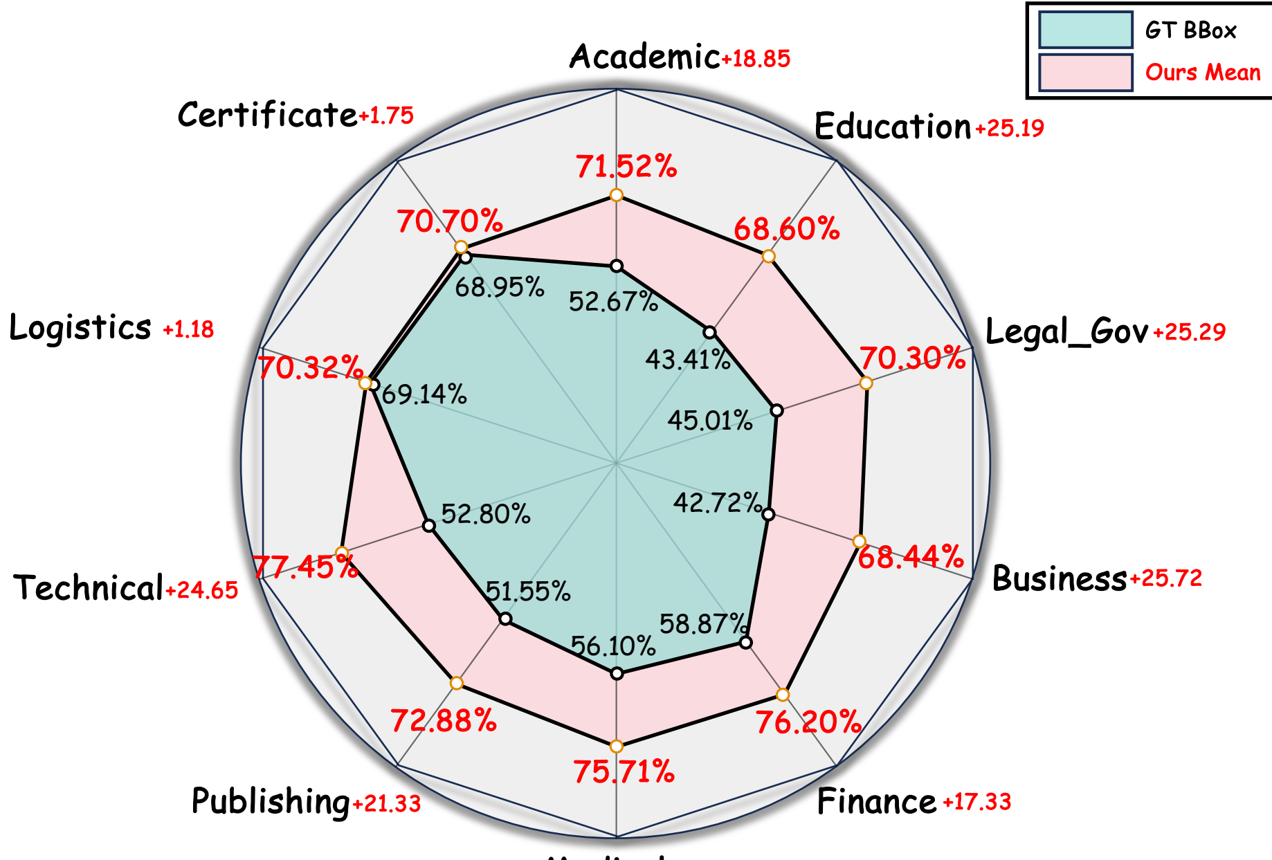
PureDocBench
