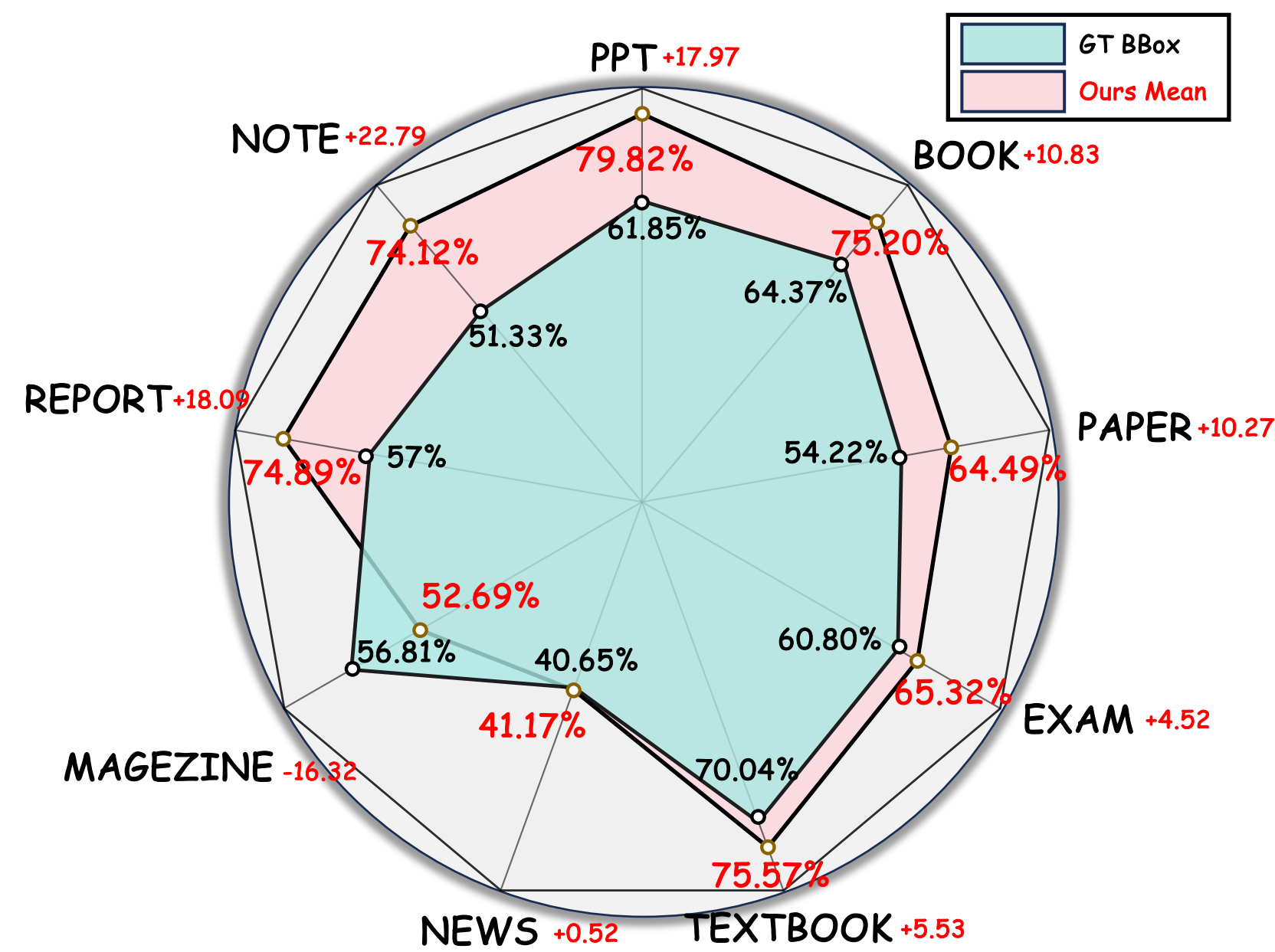
OmniDocBench v1.6
