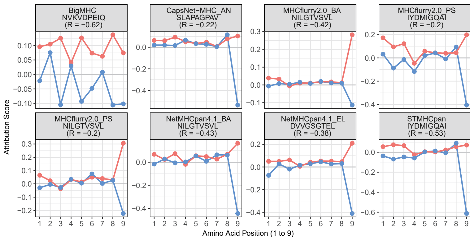
Peptide-Level Examples of SHAP vs LIME Disagreement
