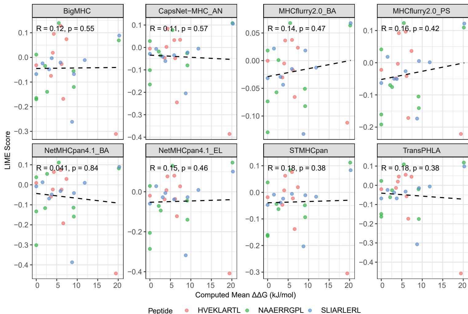
LIME: Correlation between Computed \Delta\Delta G and Attribution Score
