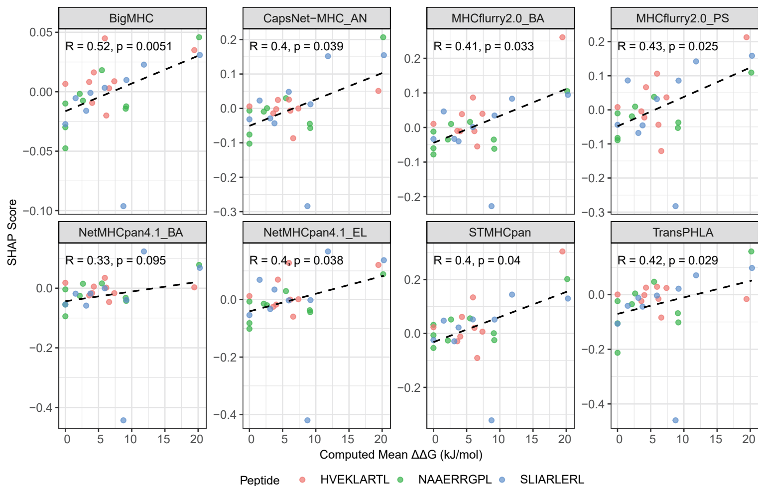
SHAP: Correlation between Computed \Delta\Delta G and Attribution Score
