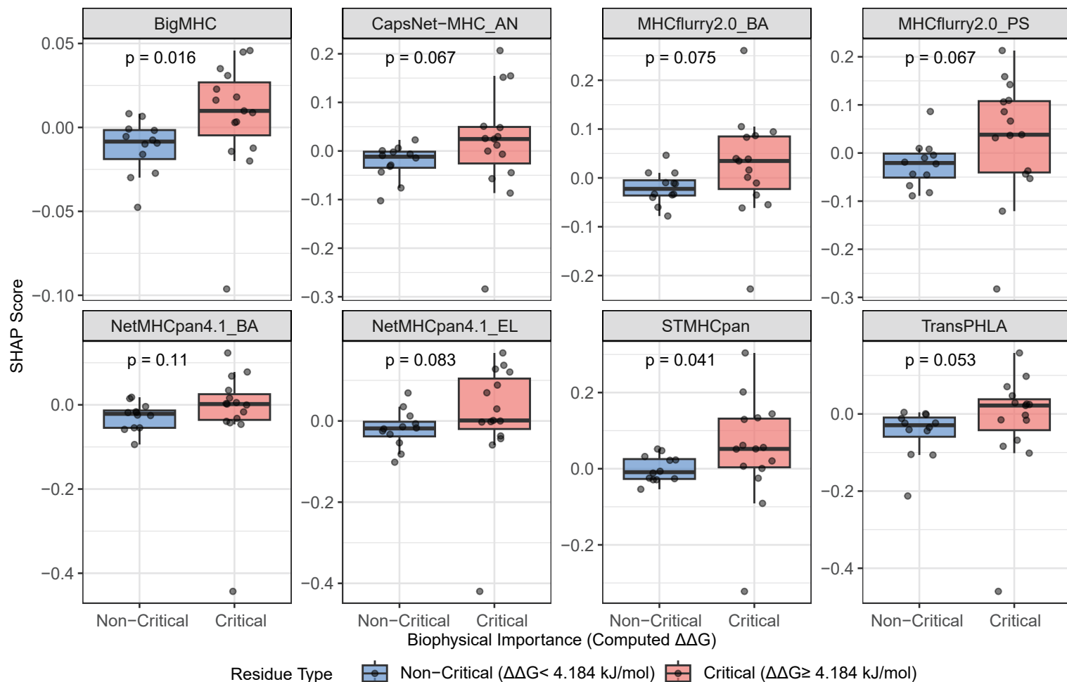
SHAP: Attribution Score Distribution by Energetic Importance
