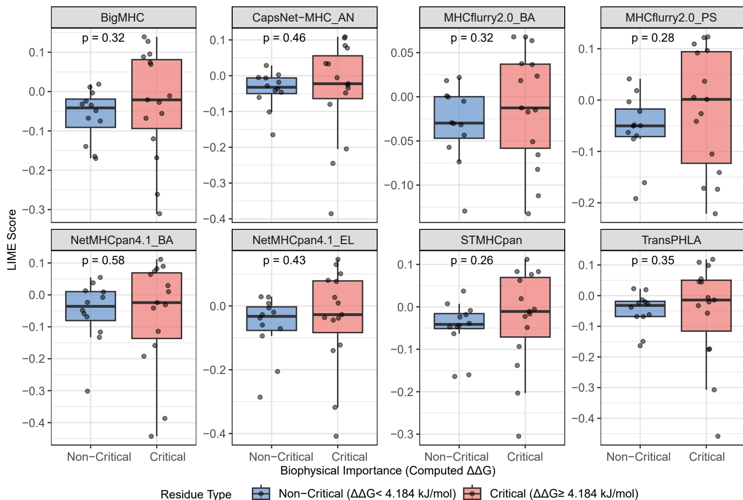
LIME: Attribution Score Distribution by Energetic Importance
