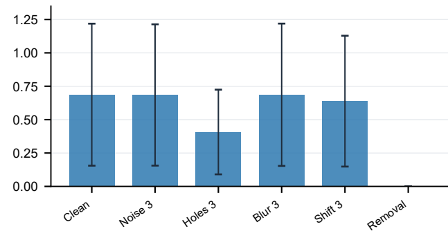
Depth selected
