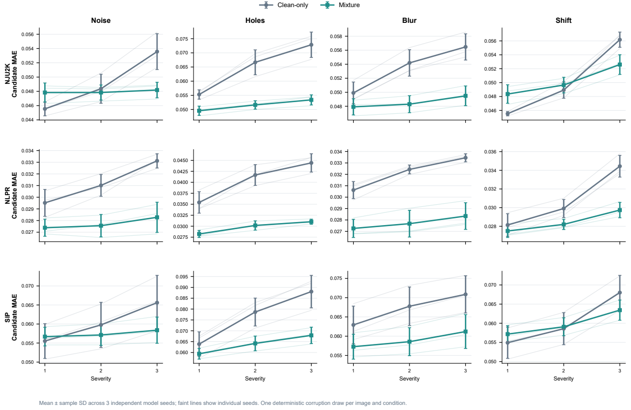
Figure 3: Candidate MAE under four depth-degradation families and three severities on NJU2K, NLPR, and SIP. Curves compare clean-only and corruption-mixture candidate training; bold points and error bars are the mean \pm sample SD across three model seeds, and faint lines show individual seeds. Each image, condition, and seed has one deterministic perturbation realization. Complete removal is reported separately in Table 4.
