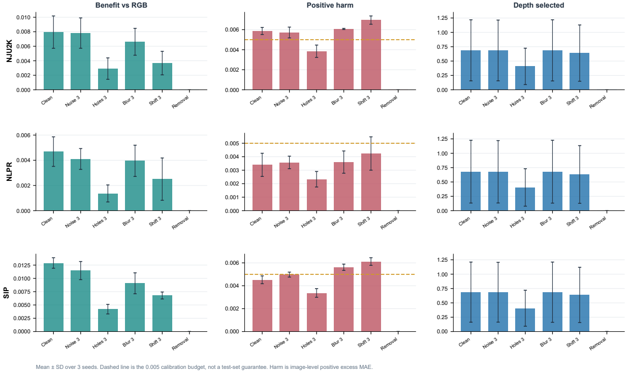
Figure 4: Held-out test diagnostics for the calibrated router. Each bar is the three-seed mean and each error bar the sample SD. Benefit is RGB MAE minus routed MAE; positive harm is the mean positive image-level excess MAE relative to RGB; depth selected is the fraction of regions using the RGB-D candidate. The dashed 0.005 line denotes an empirical calibration budget only. The plotted conditions are clean, severity 3 for each corruption family, and removal.
