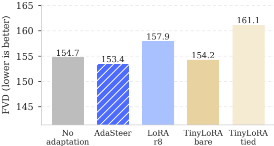
Panda-70M, 999 videos
