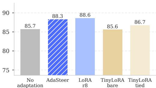
UCF-101, 932 videos
