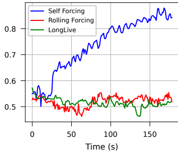
Share of rollouts frozen (1 s windows)
