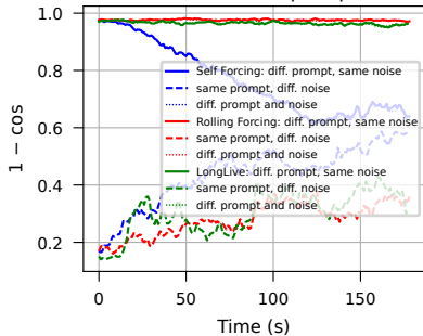
Who decides the future: prompt or noise?
