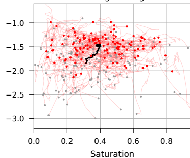
Ensemble spread of saturation
