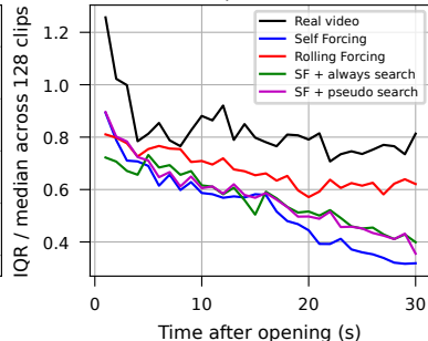
Ensemble spread of saturation
