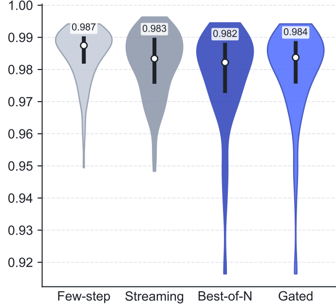
Temporal flickering (higher = steadier)
