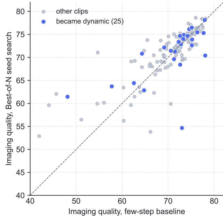
(a) Picture quality, clip by clip
