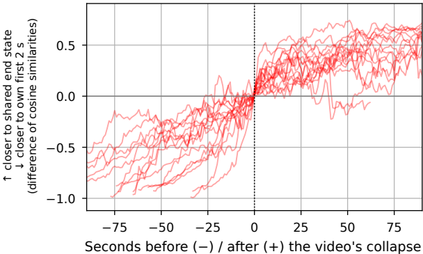
(a) 16 Self Forcing videos, aligned at collapse
