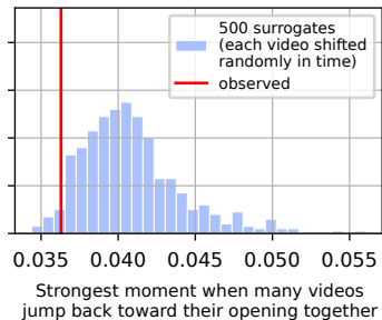
LongLive ( p = 0.97 )
