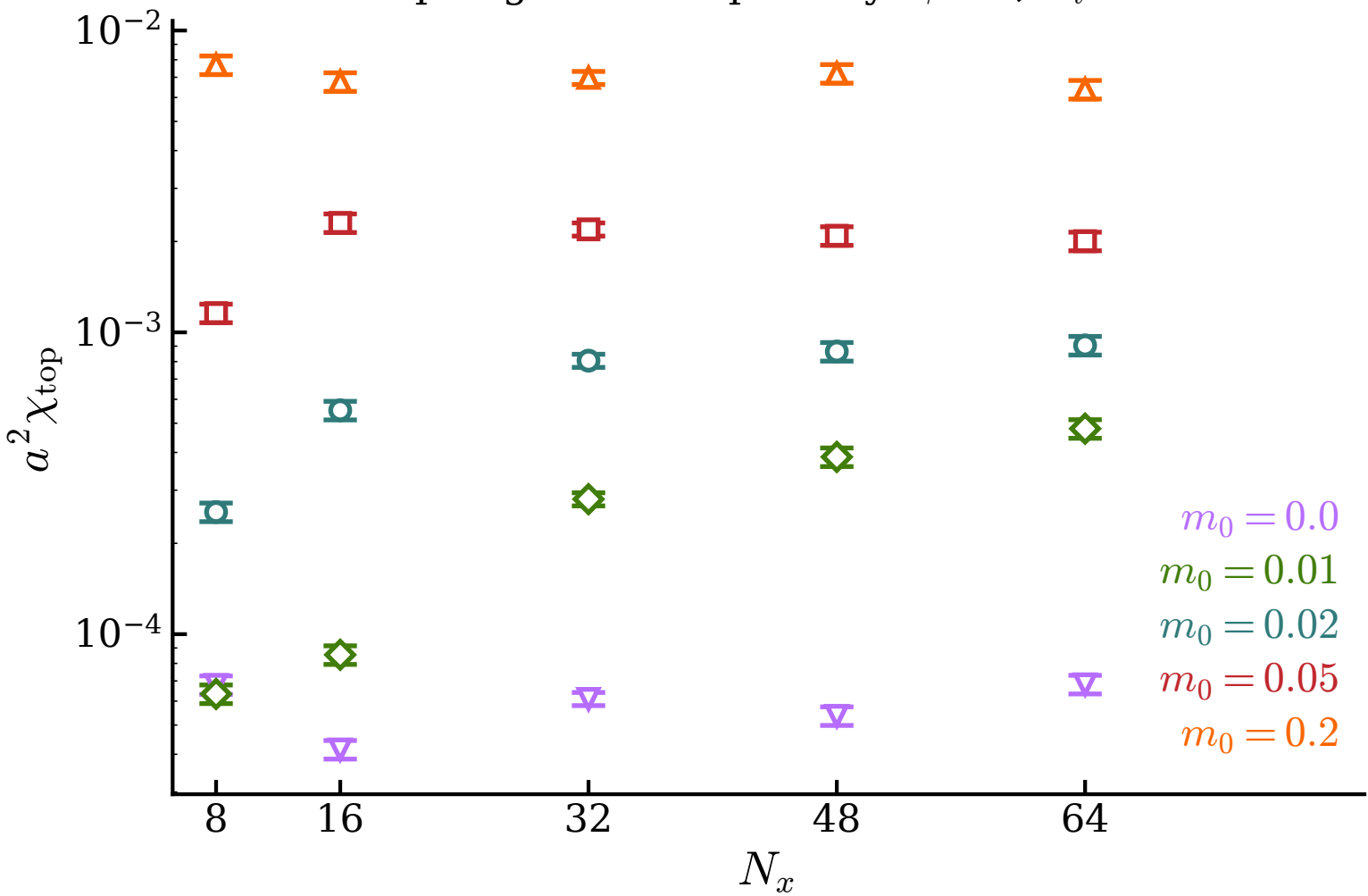
Topological susceptibility: \beta = 3 , N_t = 64
