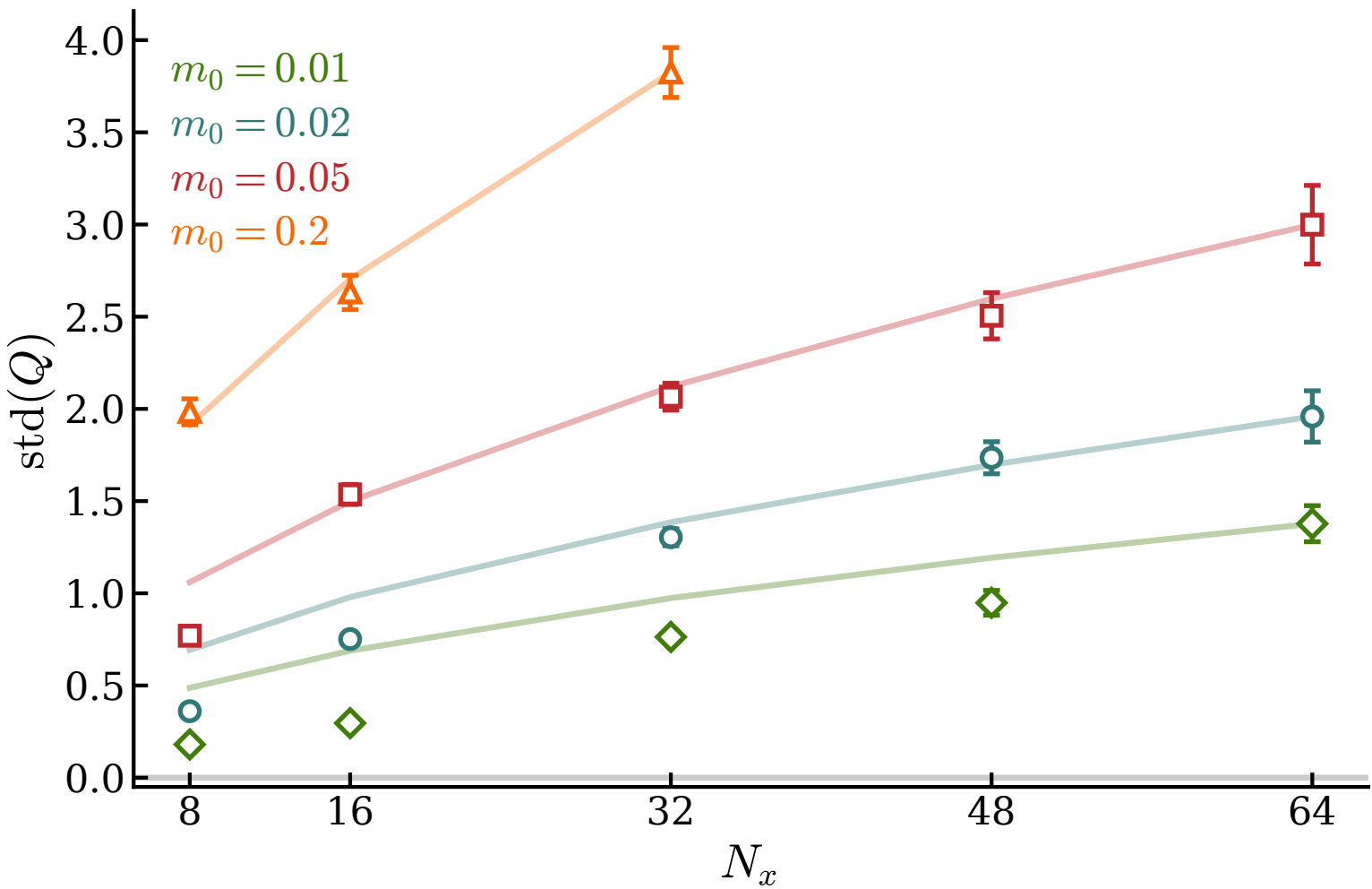
Topological charge sampling: \beta = 3 , N_t = 64
