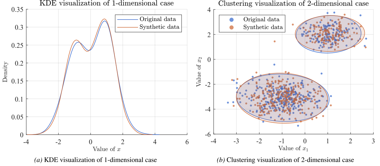
Figure 3. Comparison of original and synthetic data. (a) Kernel Density Estimations (KDE) for the 1-dimensional case. (b) Clustering results for the 2-dimensional case.
