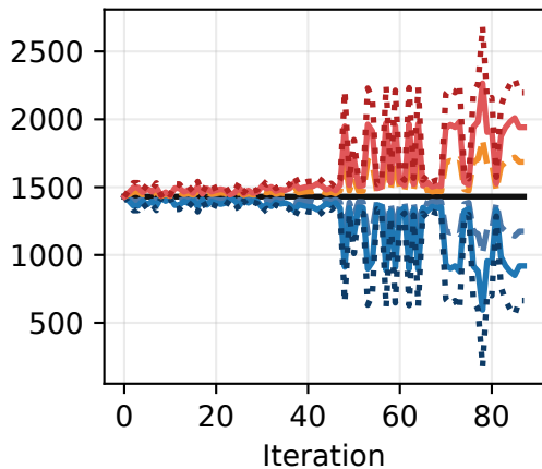
32B Reference-Based Drift
