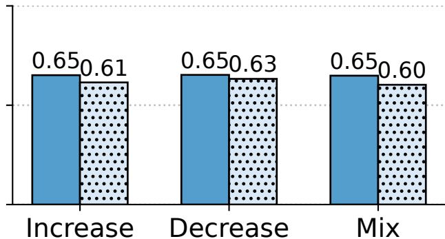
Train Utilization
