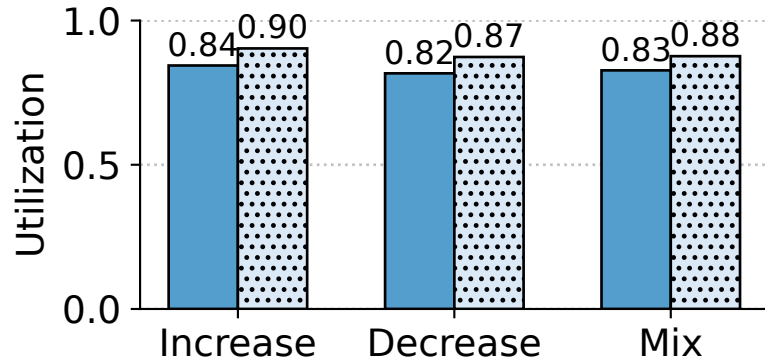
Rollout Utilization
