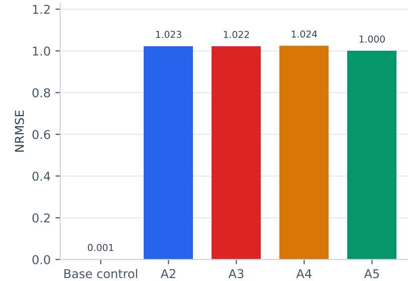
Normalized RMSE
