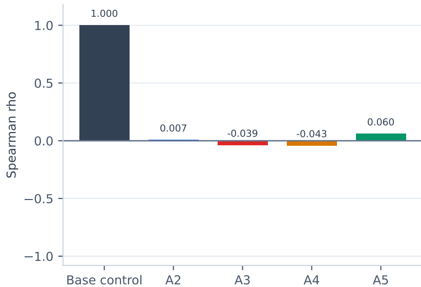
Absolute-weight ranking
