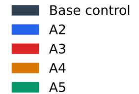
Evaluated model
