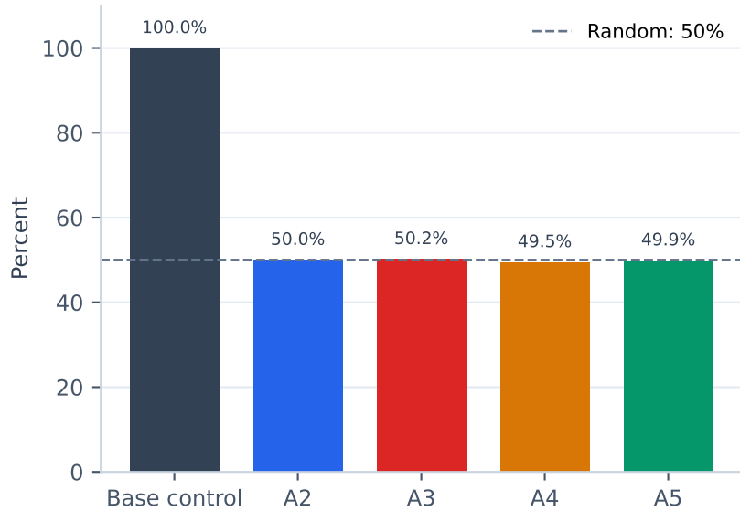
Absolute-weight ranking
