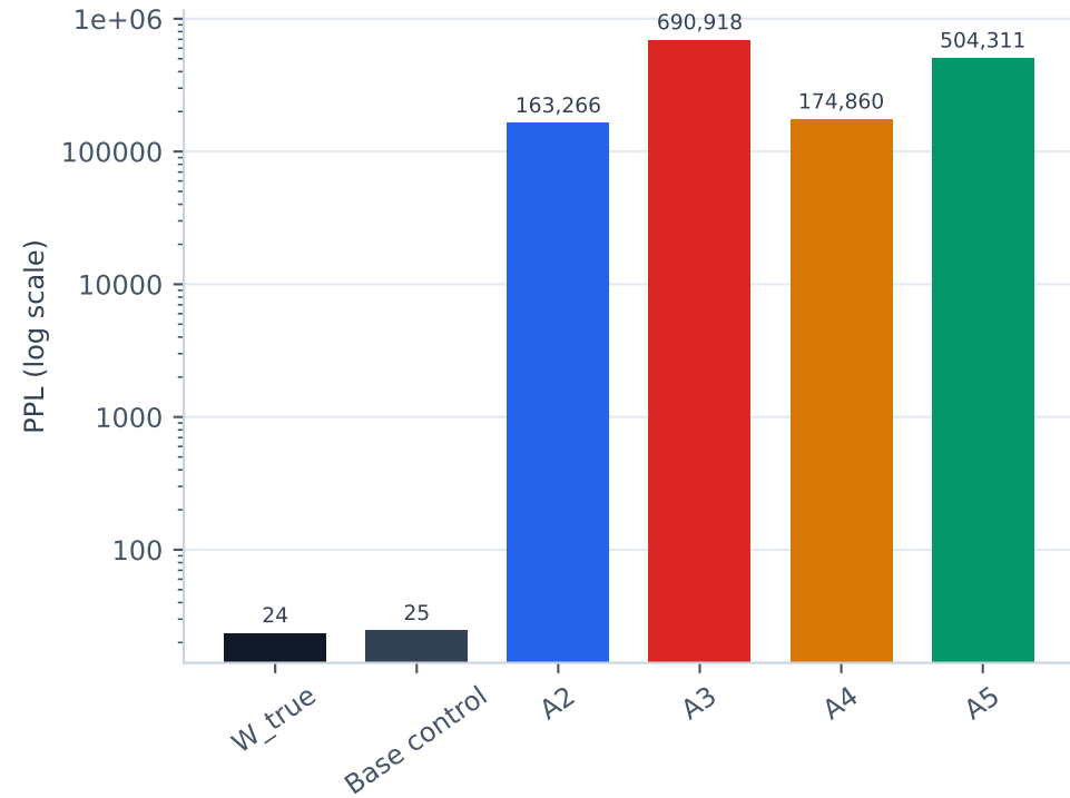
Perplexity
