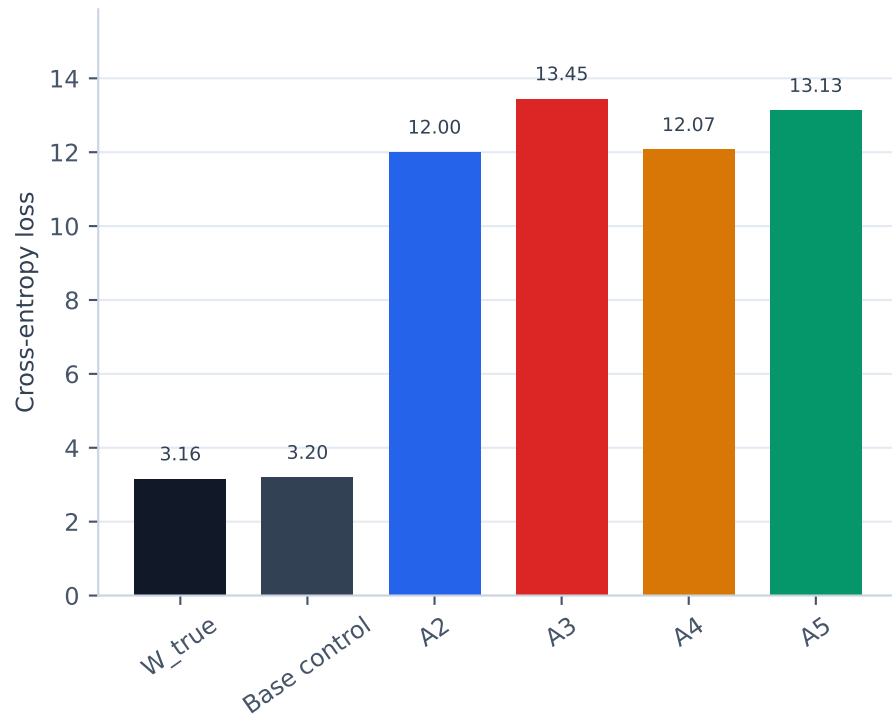
Validation loss
