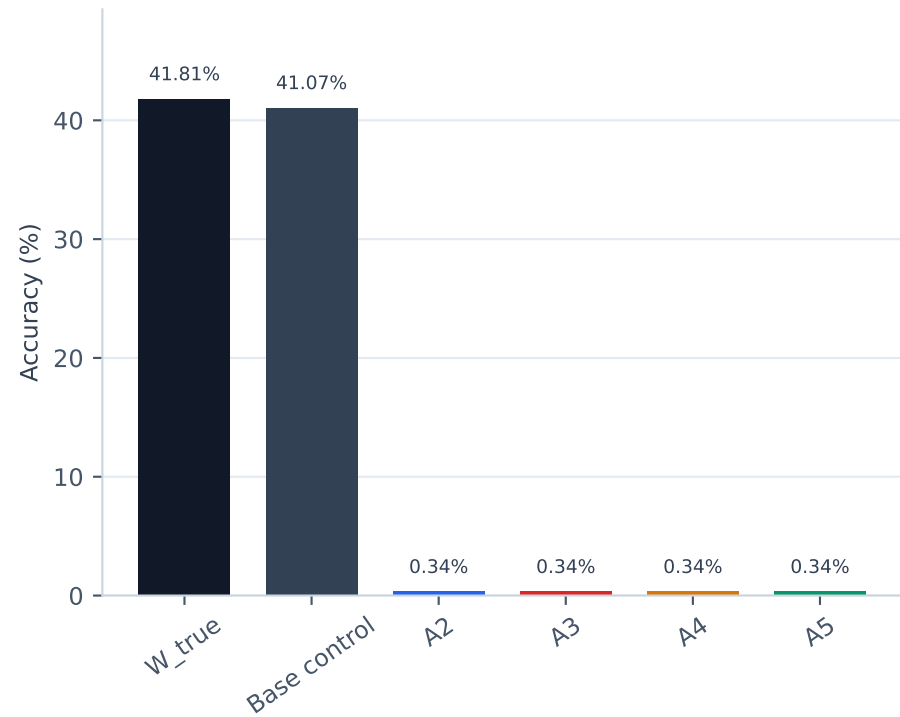
Next-token accuracy
