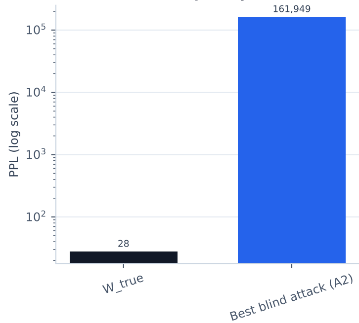
Perplexity
