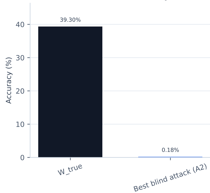
Next-token accuracy
