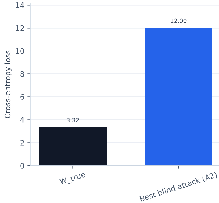
Validation loss
