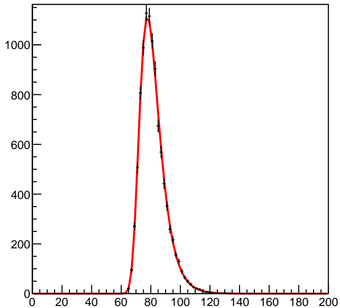
Gumbel Distribution
