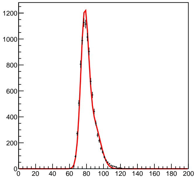
Double Gaussian
