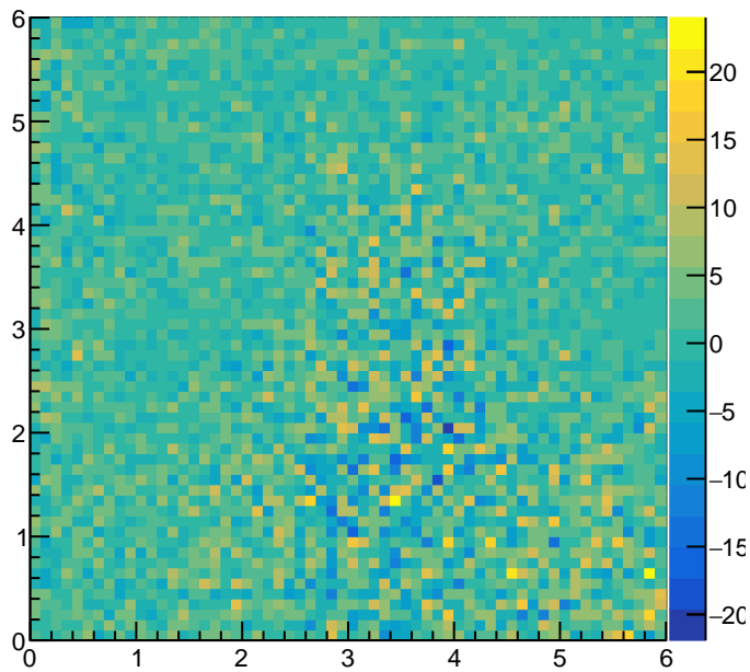
residuals
