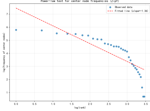
(a) Central node occurrences
