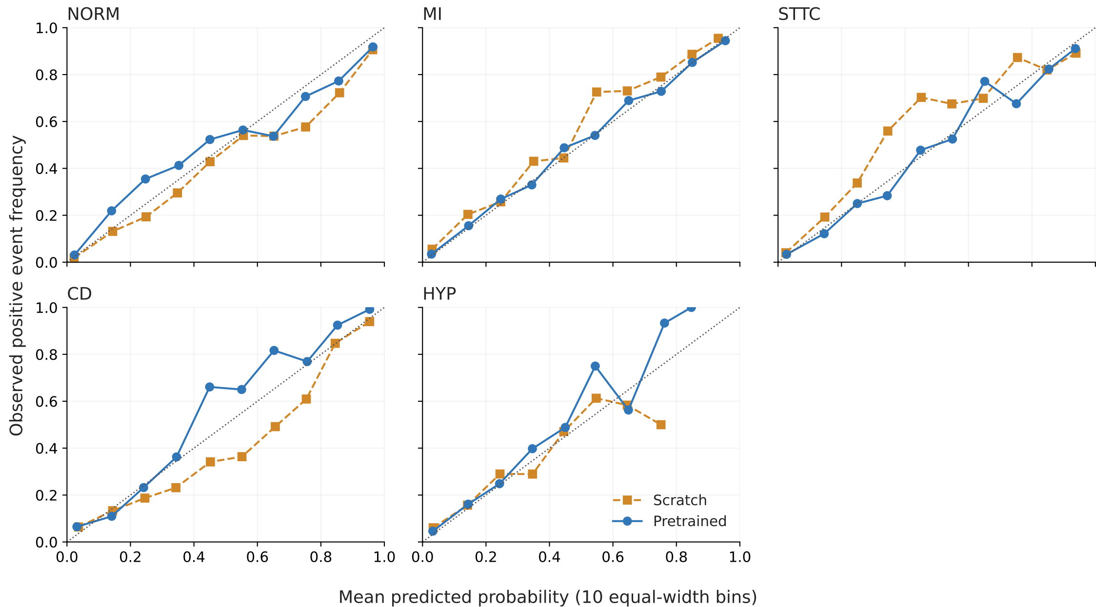
Per-class calibration | 10% labels, seed 42, PTB-XL fold 10
