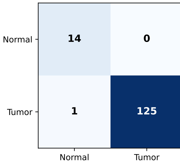
SVM_RBF
