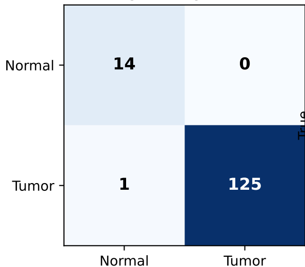
XGBoost
