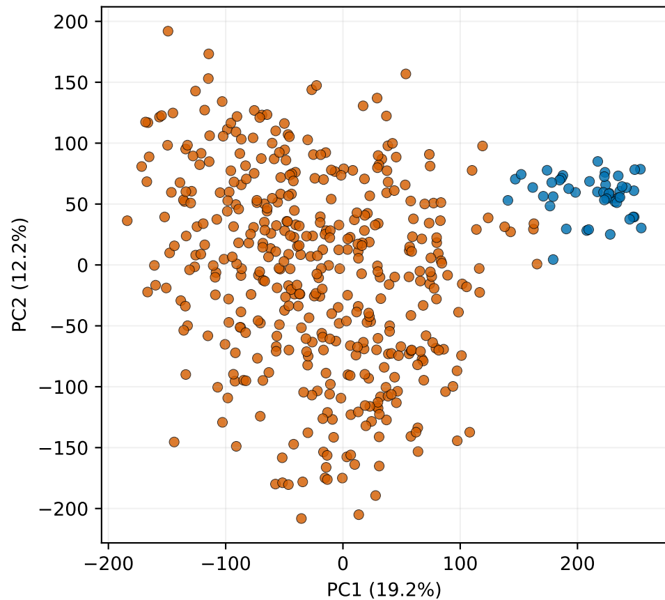
After ComBat
