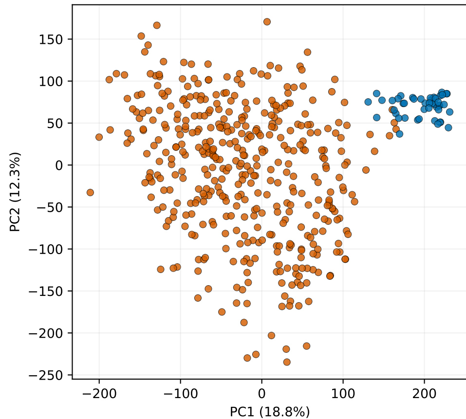
Before ComBat
