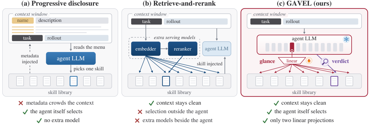
Figure 1 | Three designs for skill routing. (a) Progressive disclosure preloads every skill’s metadata into the prompt, crowding the context. (b) Retrieve-and-rerank keeps the context clean but hands selection to external models that never see the rollout. (c) GAVEL routes with the frozen agent LLM itself: a glance over the whole library, read from one mid-layer state through two trained linear maps, then a verdict in which the same model examines the top candidates in full.
