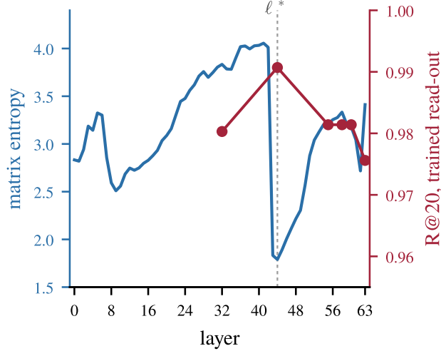
Figure 7 | Selecting \ell^* . Left axis: matrix-based entropy of the token states of a rendered skill, median over 500 skills, sink token removed. Right axis: R@20 of the read-out trained at each of six candidate depths, on the validation queries. The trained scan peaks at the entropy floor the unsupervised criterion picks.
