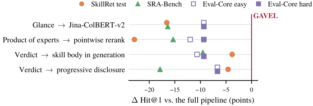
Figure 4 | Ablations. Each row replaces one design choice of GAVEL and shows how far the full pipeline drops on each benchmark, in points against the unmodified router (red line). On Eval-Core the hollow marker is the easy pool and the filled one the hard pool.
