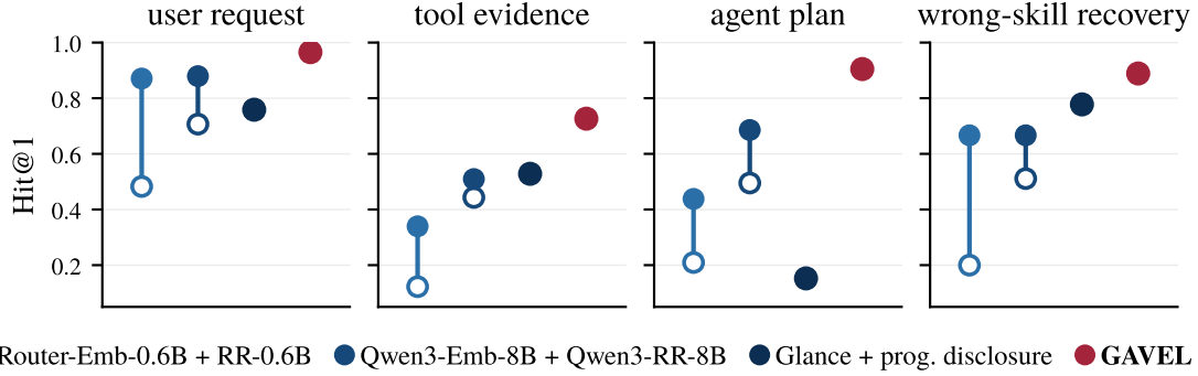
Figure 5 | Routing mid-rollout on SkillTraj, a panel per scenario. A retrieve-and-rerank pipeline has two points, hollow when it swallows the full trajectory, filled when it keeps only the last message.
