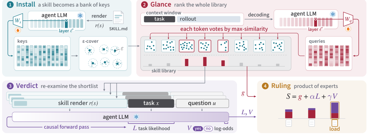
Figure 2 | The GAVEL pipeline. Install : W_s maps a new skill’s layer- \ell^* states in the frozen agent LLM to a bank of keys thinned by an \epsilon -cover. Glance : W_q reads the same layer as the model decodes; each task token votes by max-similarity over every bank, ranking the whole library. Verdict : the model re-examines each shortlisted skill against the task, giving the task likelihood L and the yes/no log-odds V . Ruling : a product of experts over glance and verdict picks the skill to load.
