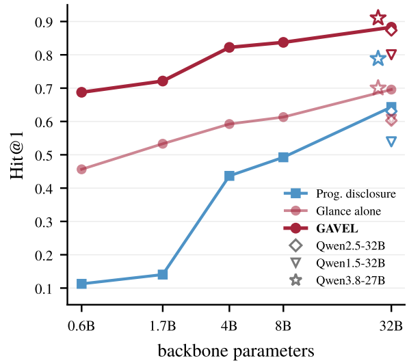
Figure 6 | Routing accuracy on SRA-Bench as the backbone grows more capable, across Qwen3 sizes (solid lines), across generations at a fixed 32B (hollow markers), and onto Qwen3.8-27B (stars).
