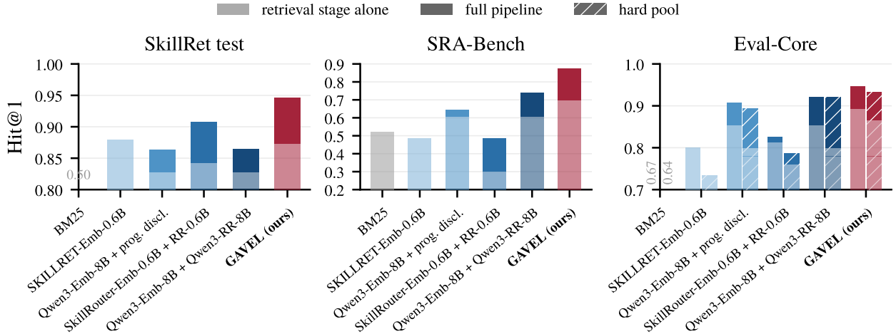
Figure 3 | Routing from written tasks. Light fill is the retrieval stage committing its top-1 alone, dark fill the full pipeline built on it, and on Eval-Core the hatched bar is the hard pool. Where BM25 falls below the plotted range its score is printed in place of the bar.
