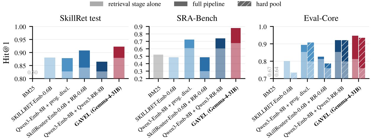
Figure 8 | The comparison of Figure 3 with the routing backbone changed to Gemma-4-31B. The baselines do not involve that backbone, so their bars carry over from Figure 3; the rebuilt parts are GAVEL itself and the in-context picker of progressive disclosure. Bars read as before, light fill for the retrieval stage alone, dark fill for the full pipeline, hatched for Eval-Core’s hard pool, and a below-range BM25 score printed in place of its bar.
