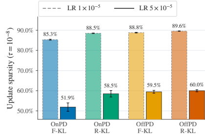
Figure 18: Parameter-update sparsity with a smaller threshold. Each bar pools the three datasets and N = 3 repeats per dataset; error bars show SEM across the nine runs. Learning rate, more than rollout policy, determines sparsity of updates.
